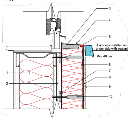
Diagram 7 - Typical window over cill detail
