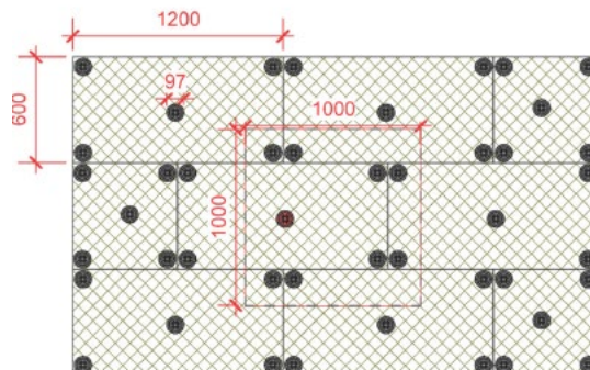
Diagram 2 - Typical fixing pattern (5 fixings per board or 8 fixings per m 2 )
