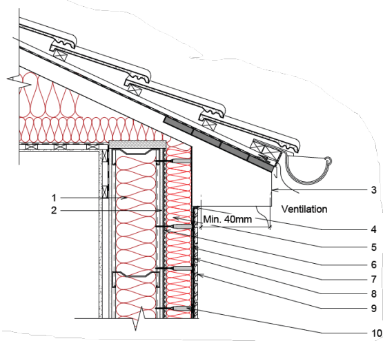
Diagram 3 - Typical overhanging eaves detail
