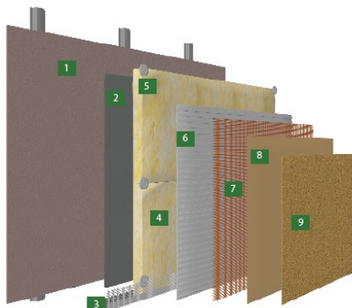
Diagram 1 - Typical build up fixed through MW only - with silicone render
