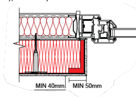
Diagram 8 - Typical window jamb detail
