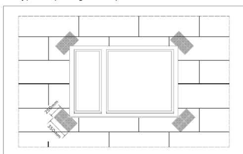
Diagram 9 - Typical opening stress patch detail
