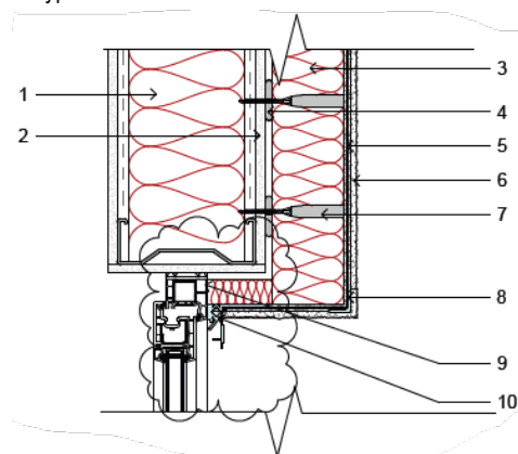
Diagram 6 - Typical window head detail
