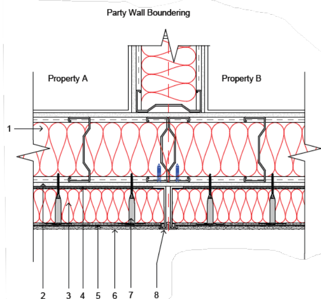
Diagram 4 - Typical vertical movement joint detail
