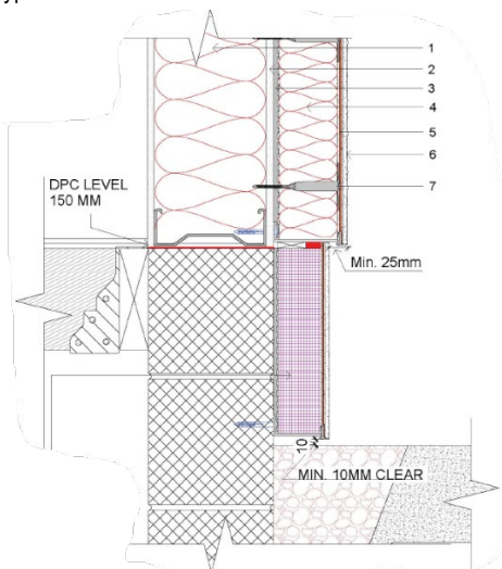
Diagram 5 - Typical standard base detail
