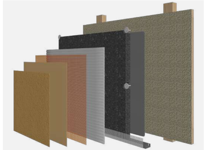
PARK HOME - RENDER ONTO RENDER CARRIER BOARD
