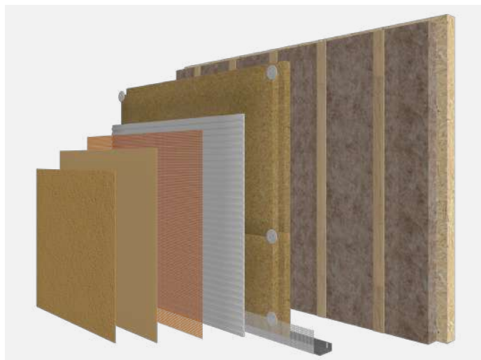
RENDER ONTO WOOD FIBRE INSULATION
