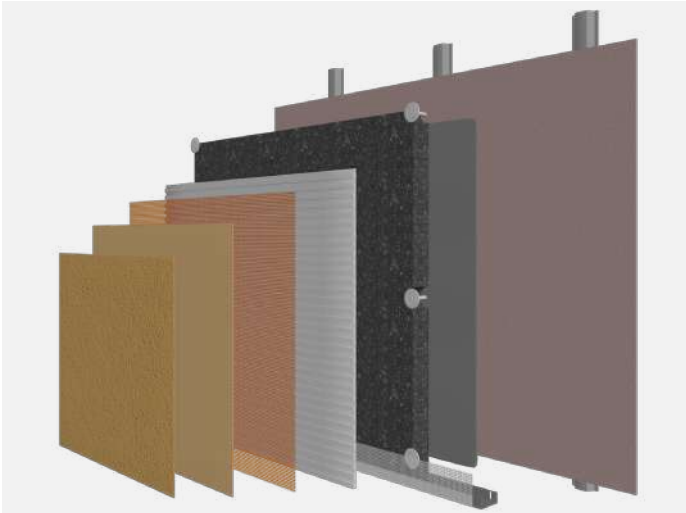
EPS ONTO RENDER CARRIER BOARD
